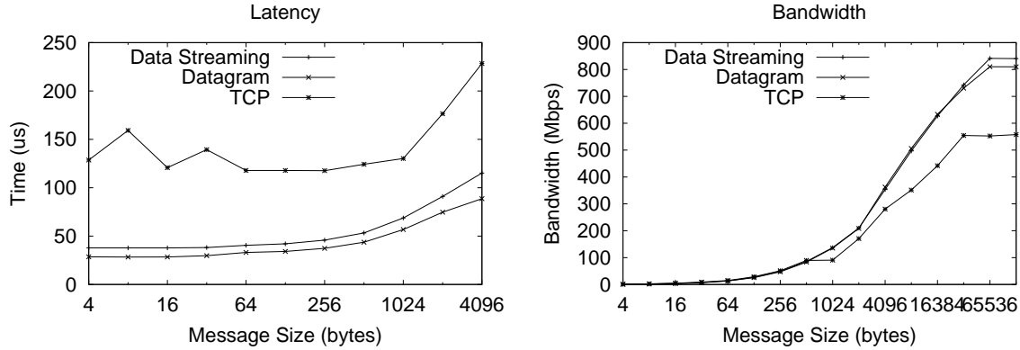
Figure 13: Micro-Benchmarks Results
