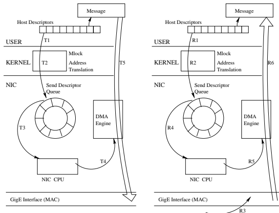
Figure 2: EMP protocol architecture showing operation for transmit (left), and receive (right).
