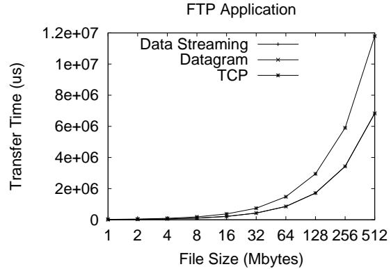
Figure 14: FTP Performance
