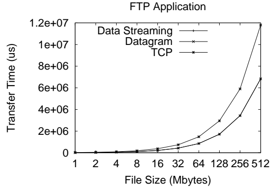
Figure 14: FTP Performance
