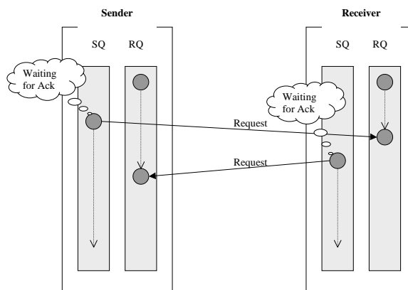
Figure 7: Deadlock in the rendezvous approach
