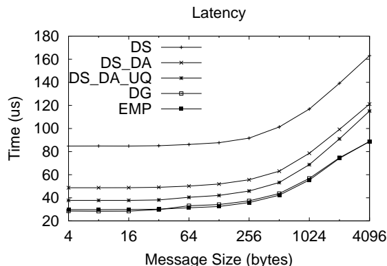
Figure 11: Micro-Benchmarks: Latency
