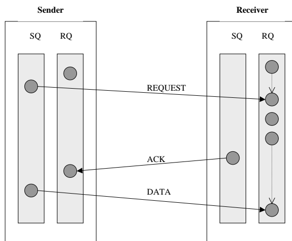
Figure 6: Rendezvous approach
