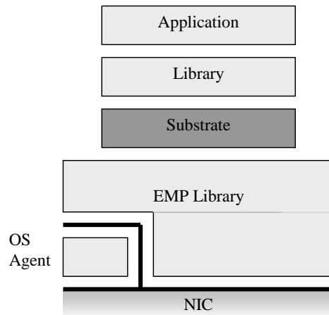
Figure 5: Sockets-over-EMP architecture
