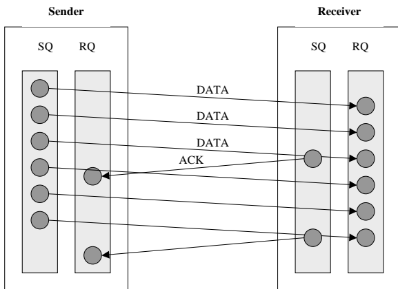
Figure 10: After Delayed Acknowledgments
