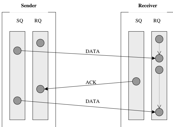
Figure 8: Eager with Flow Control
