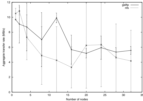
Figure 3. ROMIO perf Write Performance without Sync
