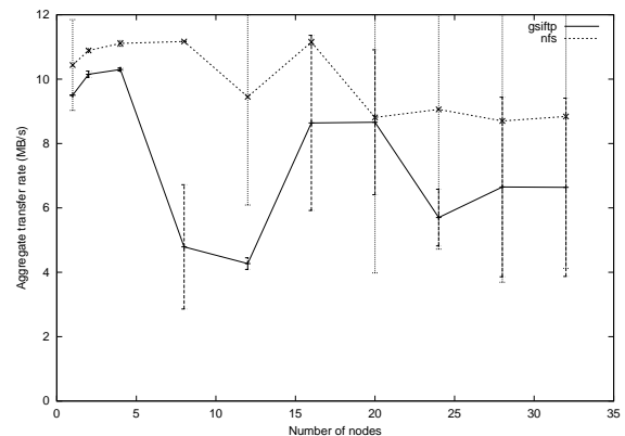
Figure 2. ROMIO perf Read Performance with Sync
