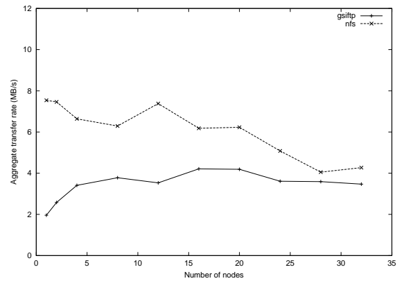
Figure 5. FLASH I/O Benchmark Checkpoint Performance using NetCDF
