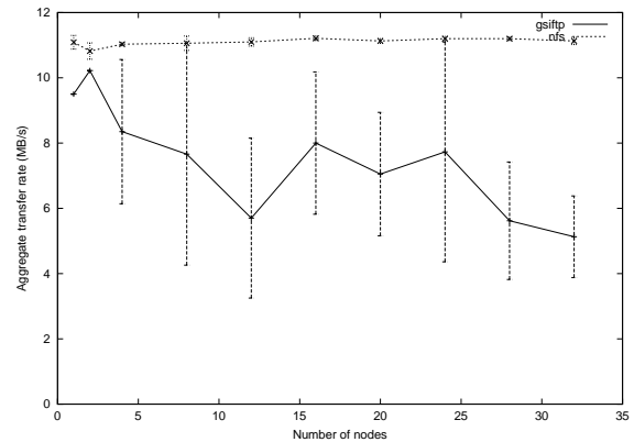
Figure 1. ROMIO perf Read Performance without Sync
