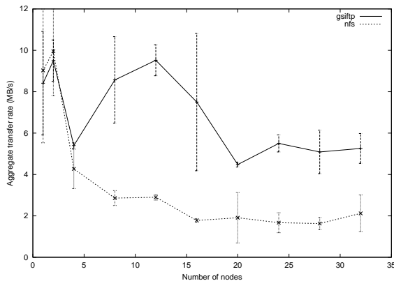
Figure 4. ROMIO perf Write Performance with Sync
