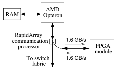
Figure 1. The Cray XD1 system
