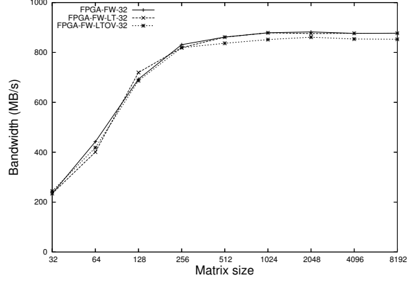
Figure 12. Measured read bandwidth from the XD1 to the FPGA kernel
