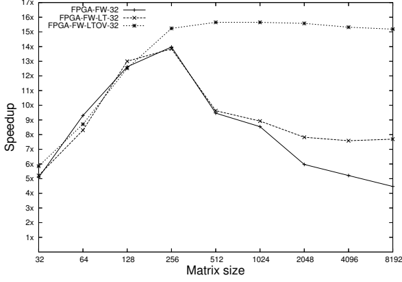
Figure 10. Measured speedup over CPU-FW-OPT
