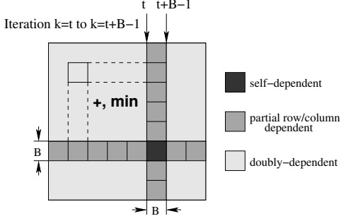
Figure 4. Tiled FW algorithm
