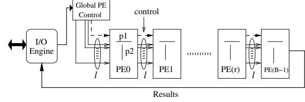
Figure 3. Parallel FW kernel architecture
