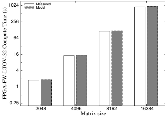
Figure 13. Measured vs. Modeled latency for FPGA-FW-LTOV-32 (Eqn.3)
