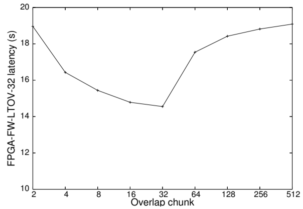
Figure 9. Optimal compute/copy overlap chunk (for 2048 nodes)
