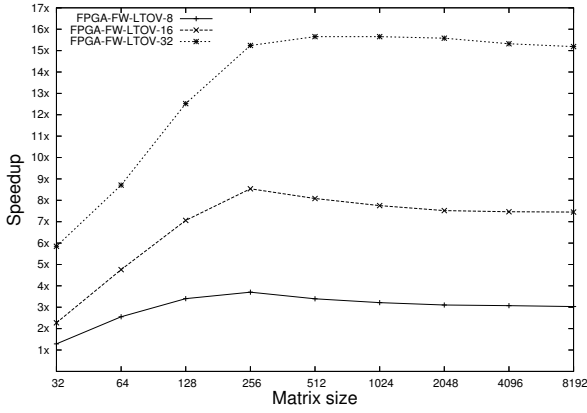
Figure 11. Performance comparison: 8x8, 16x16, and 32x32 kernels
