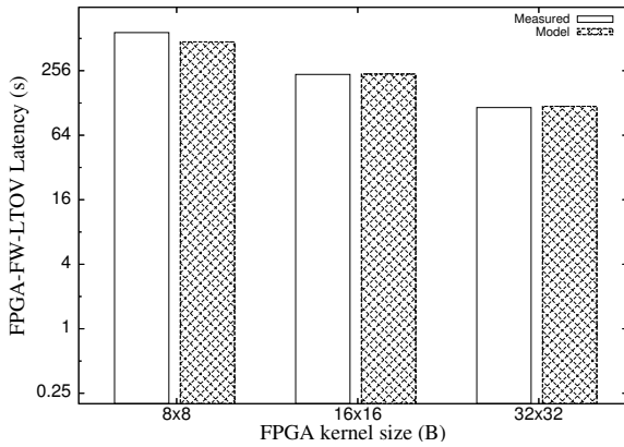
Figure 14. FPGA-FW-LTOV latency for 8192 nodes with various kernels: Measured vs. Model (Eqn. 3)
