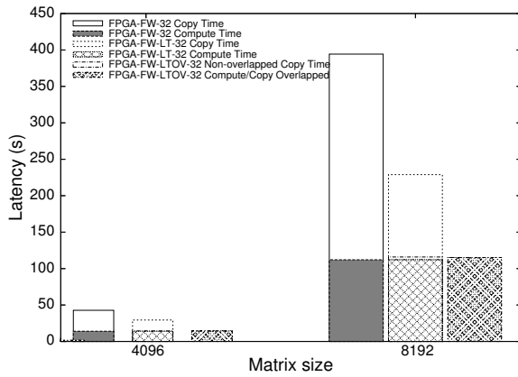
Figure 8. Copy/compute time breakdown with different optimizations
