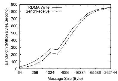
Figure 13: MPI Bandwidth Comparison
