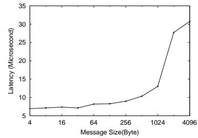
Figure 9: MPI Latency
